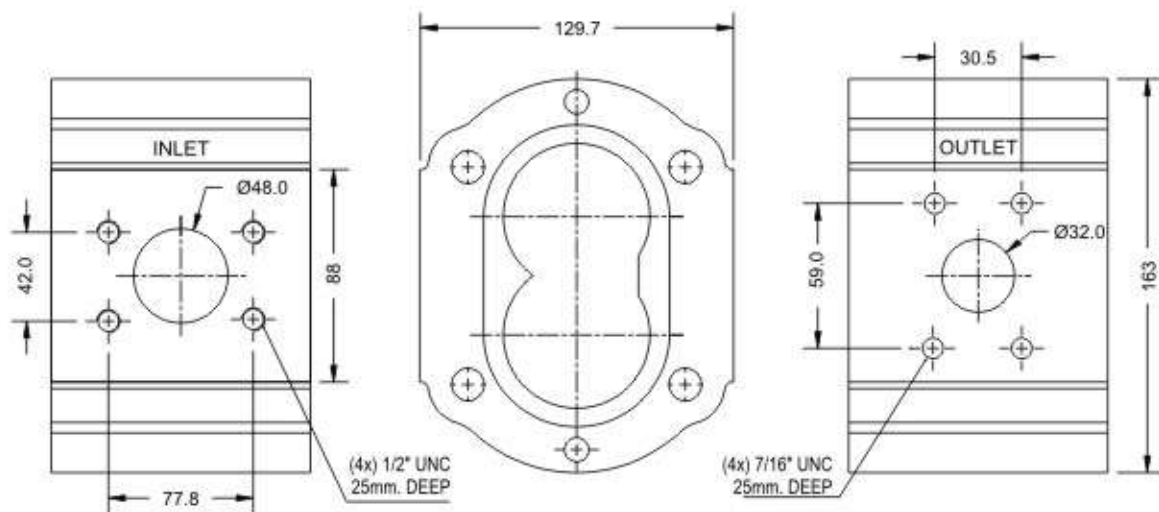
PUMP TYPE SGP-150 & SGP-173
