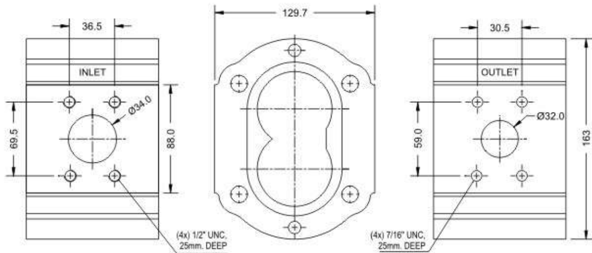
PUMP TYPE SGP-68 & SGP-136
