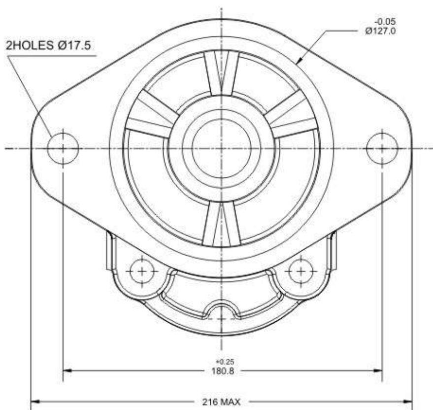
FLANGE CODE - S
