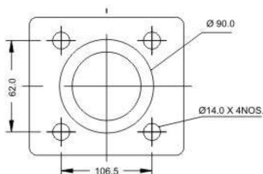
2A SGP 225 INLET SPECIAL FLANGE
