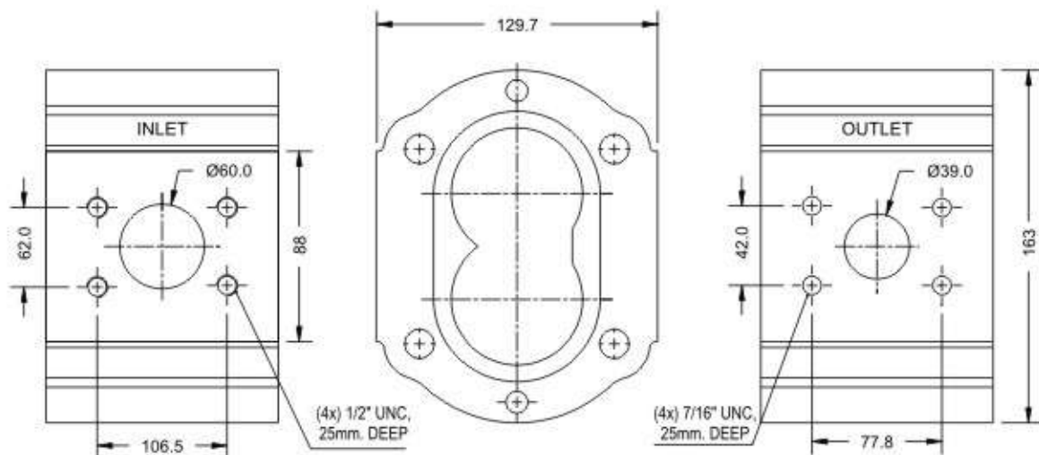
PUMP TYPE SGP-225
