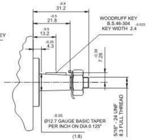
SHAFT CODE - T
